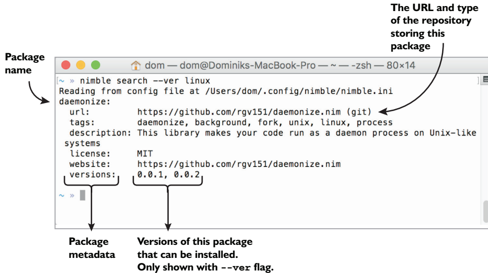
Figure 5.4 Searching for a “linux” package with version information
