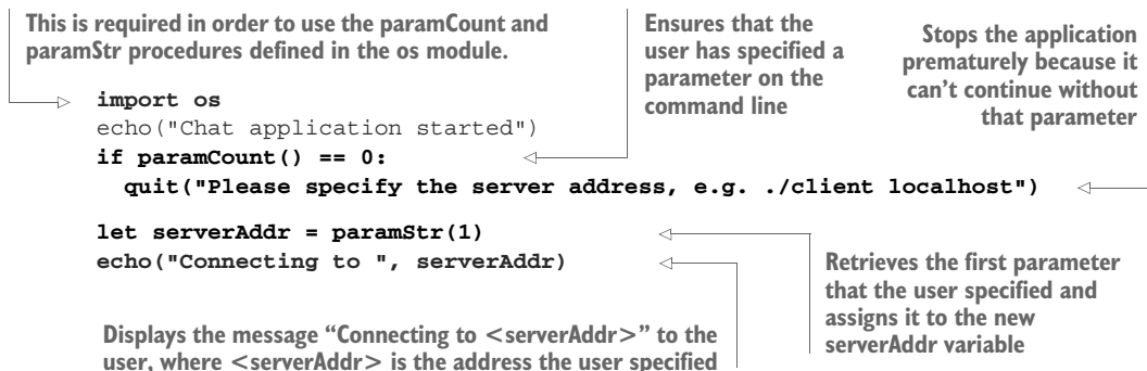
Listing 3.3 Reading command-line parameters
