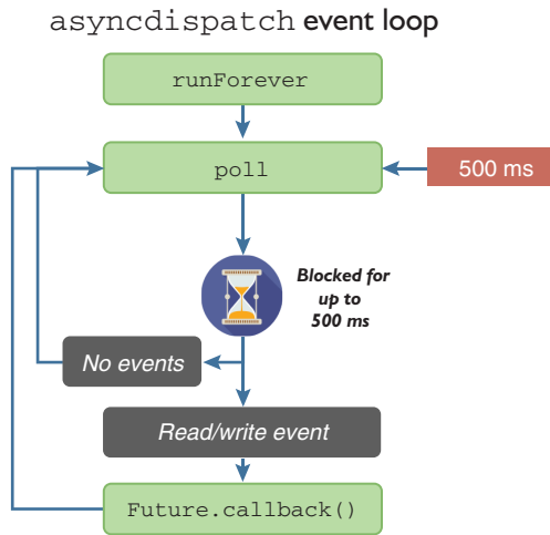
Figure 3.15 Nim's asynctdispatch event loop
