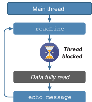
Figure 3.10 Blocking execution of client.nim
