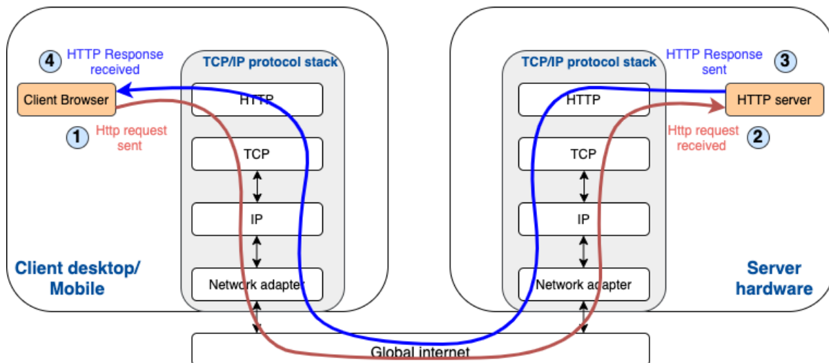
Figure 2.4 HTTP communications with protocol stack
